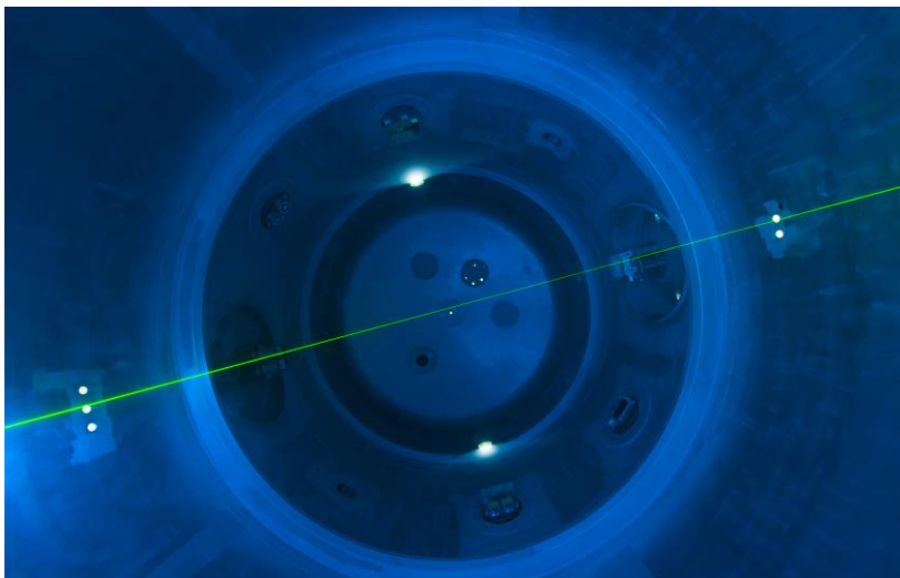
View into AIDA: Here, scientists study how dust particles influence the formation of clouds and precipitation. (Photo: Martin Lober, KIT)
