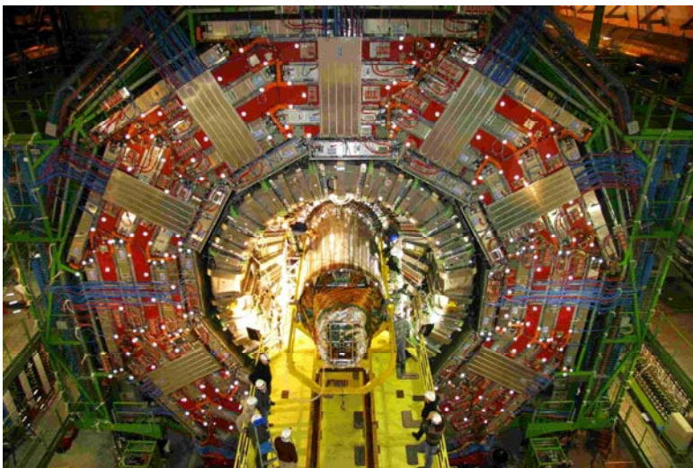
Based on the data produced by big detectors like CMS at CERN, Geneva, the structure of matter can be studied in detail. (Photo: KIT/Markus Breig)
