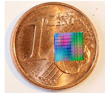
Optical chip carrying a multitude of silicon nitride microresonators (Picture: J. N. Kemal/ P. Marin Palomo/KIT)
